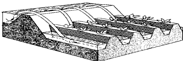
Figure: 3 Siphons on operation.
