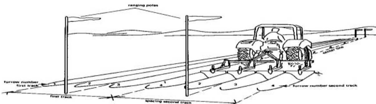
Figure.4. A ridger-drawbar behind a tractor makes four ridges simultaneously
