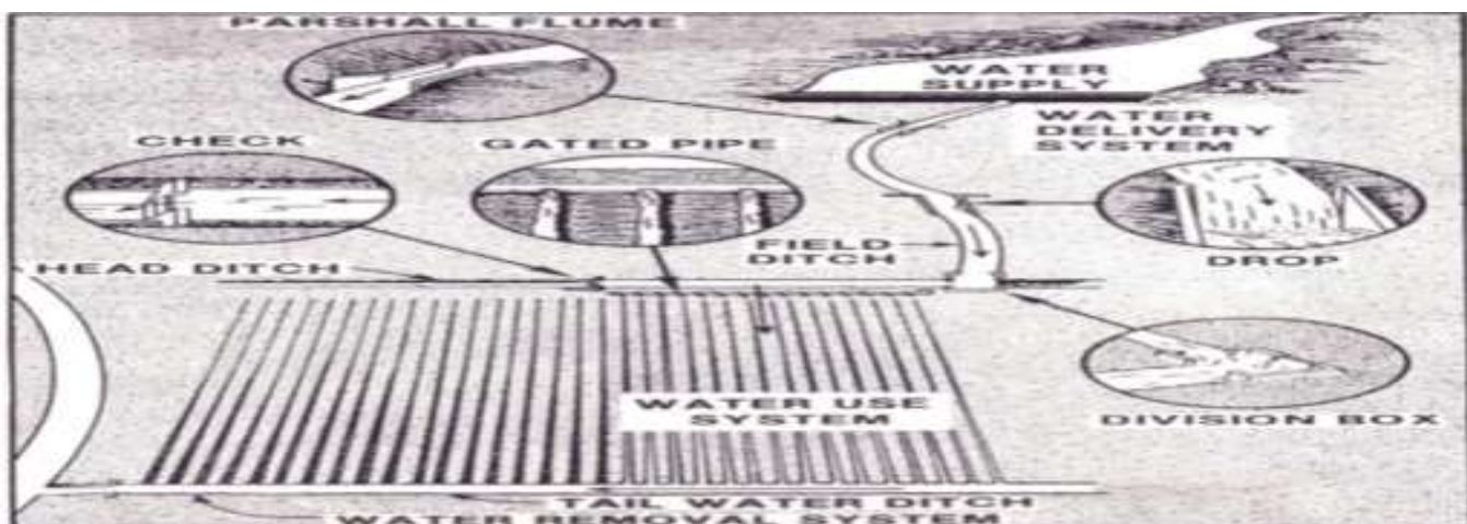
Figure: Typical elements/components of a gravity fed irrigation system. (From U.S. Department of Agriculture, Soil Conservation Service, 1967.)
